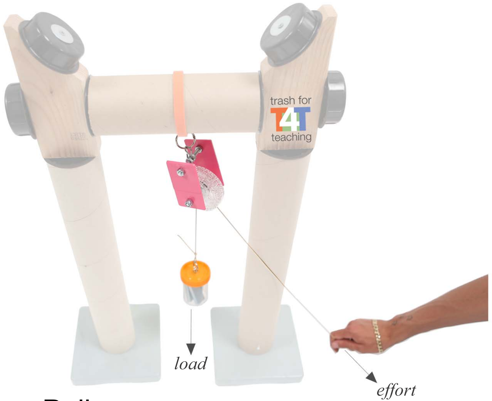
Pulley Simple Machines & Basic Forces
